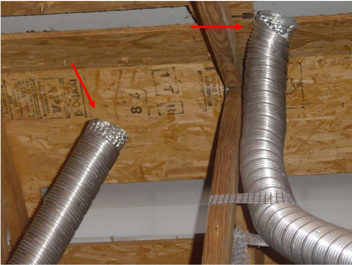
Bathroom vent pipes not discharging through the roof allowing moisture in attic
