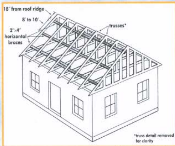
Truss Bracing
