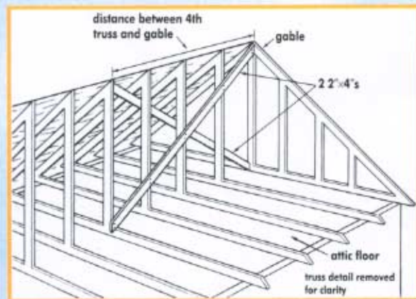
Gable End Bracing
